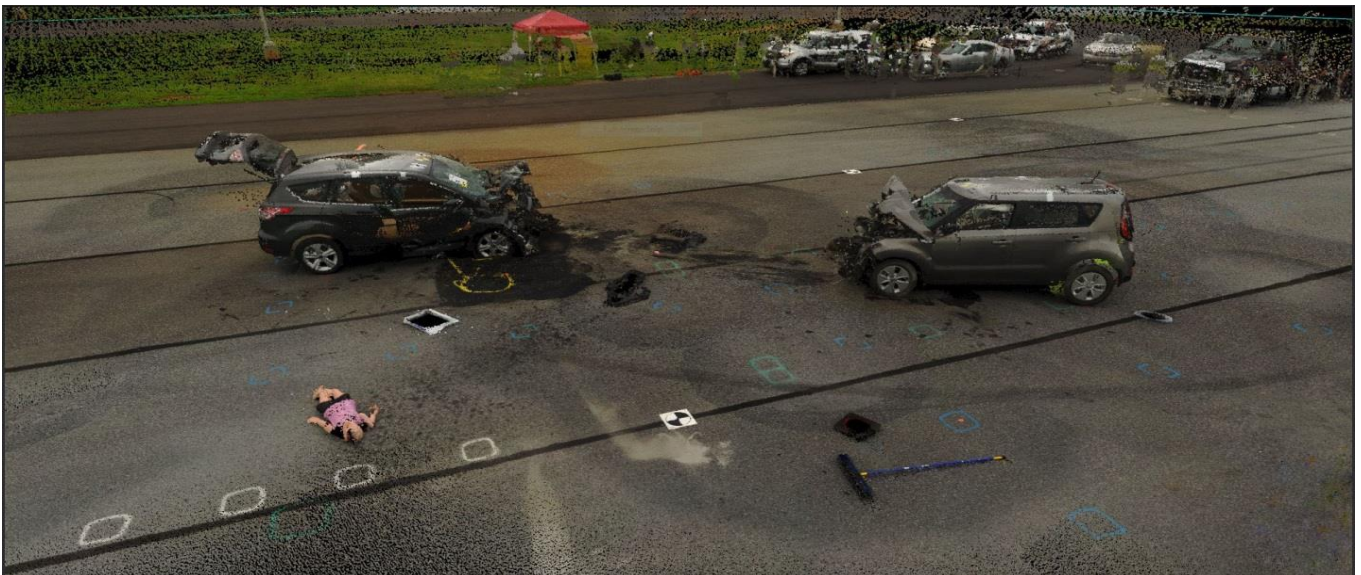
FARO System Laser Scan 3D Model Rendering
